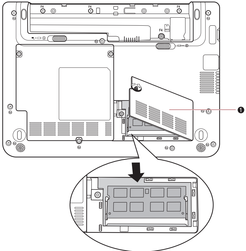
Figure 8-2 Removing the memory module cover
